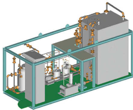
Fig3. DiaFellow™ AM outline drawing
